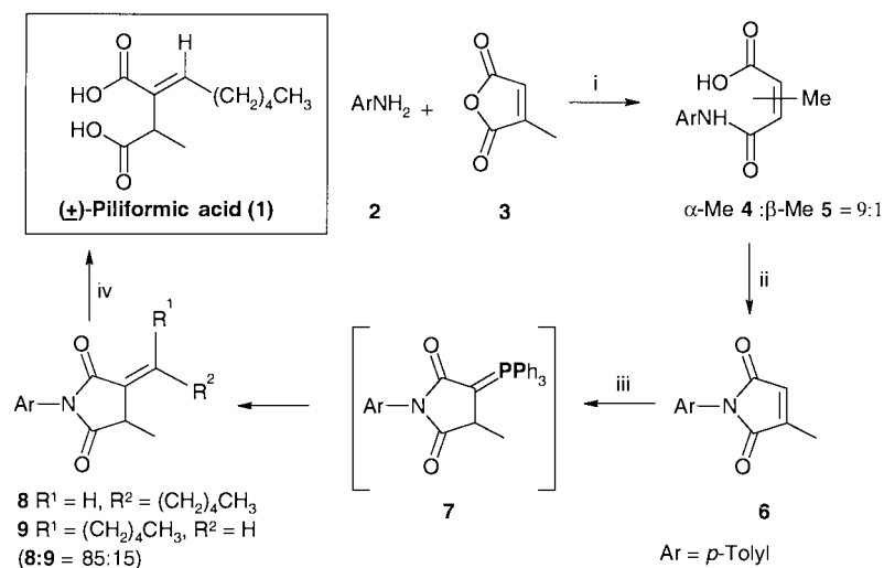
Scheme 1 Reagents, conditions and yields: (i) Et 2 O, rt, 1 h (95%); (ii) Ac 2 O–NaOAc, water-bath, 60–65 °C, 1 h (90%); (iii) TPP, AcOH, hexanal, reflux, 10 h (83%); (iv) (a) AcOH, conc. HCl, reflux, 60 h (98%); (b) recrystallisation from excess of hot water, ( E )-isomer (70%).
